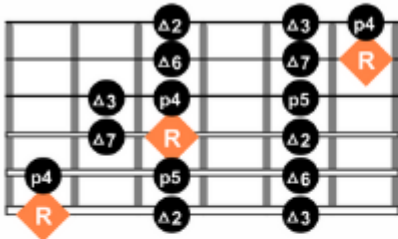
Dorian mode
