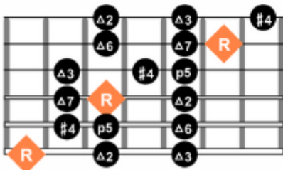
Lydian mode
