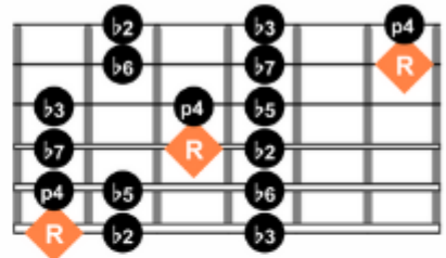
Locrian mode
