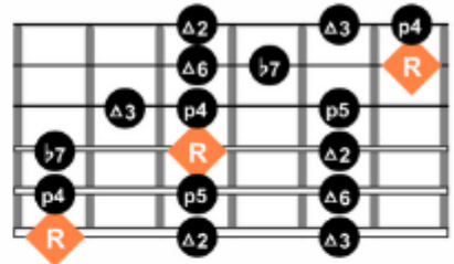
Aeolian mode
